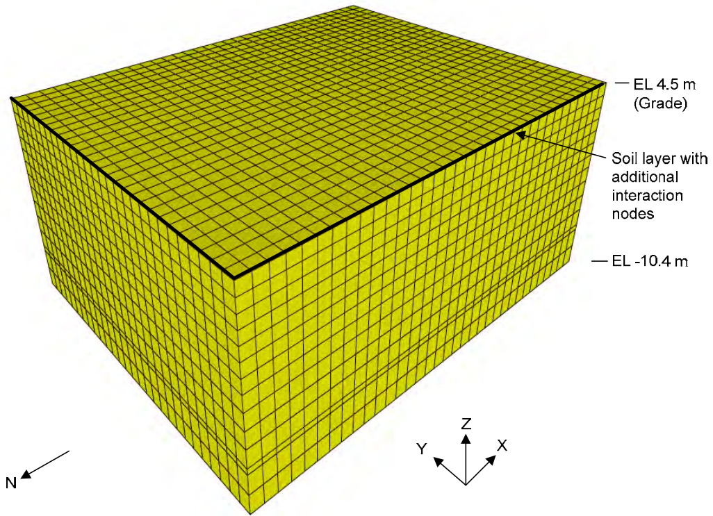
Figure 3: Excavated Soil-Rock Volume for CB MSM1 Model
