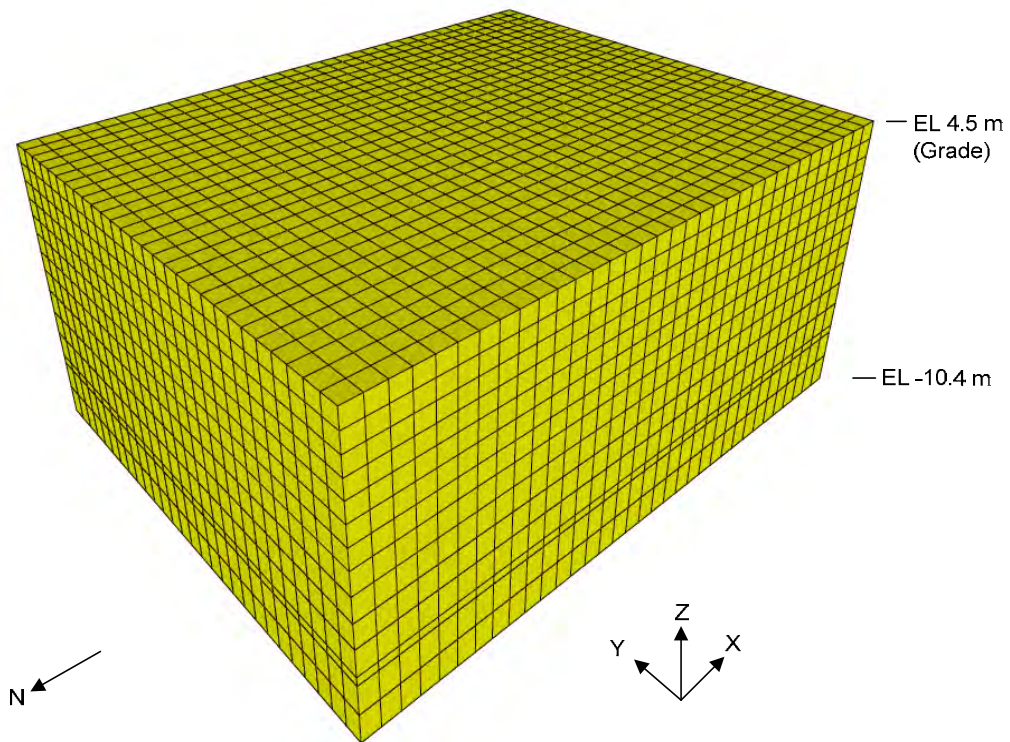
Figure 2: Excavated Soil-Rock Volume of the CB DM Model (all nodes are interaction nodes)
