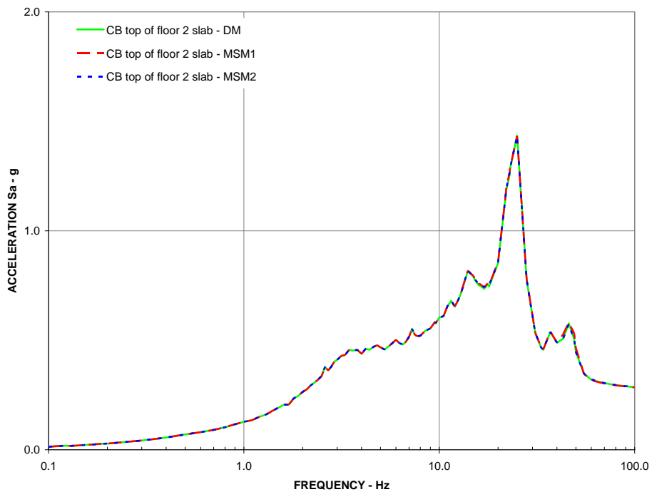
Figure 19: Z-Direction DM, MSM1, and MSM2, 5% Damped Response Spectra CB top of floor 2 (EL 4.65 m)
