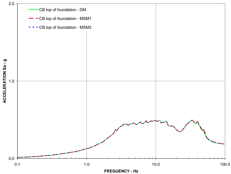
Figure 16: Z-Direction DM, MSM1, and MSM2 5% Damped Response Spectra CB top of foundation (EL -7.4 m)
