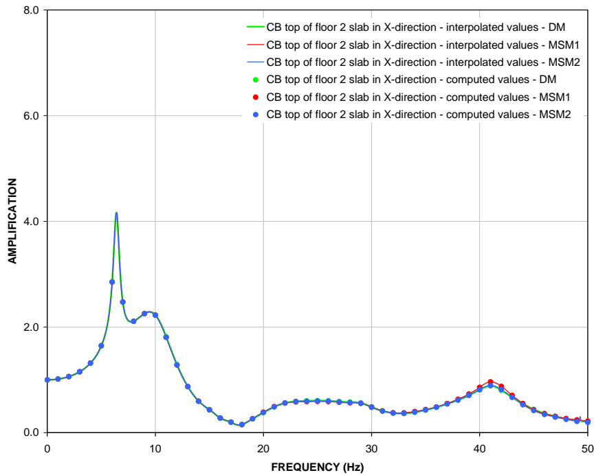
Figure 8: X-Direction DM, MSM1, and MSM2 Transfer Functions CB top of floor 2 slab (EL 4.65 m)
