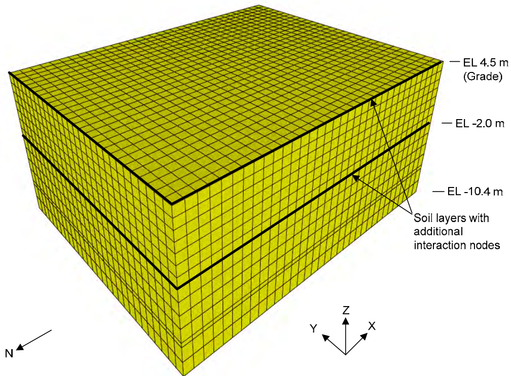
Figure 4: Excavated Soil-Rock Volume for CB MSM2 Model
