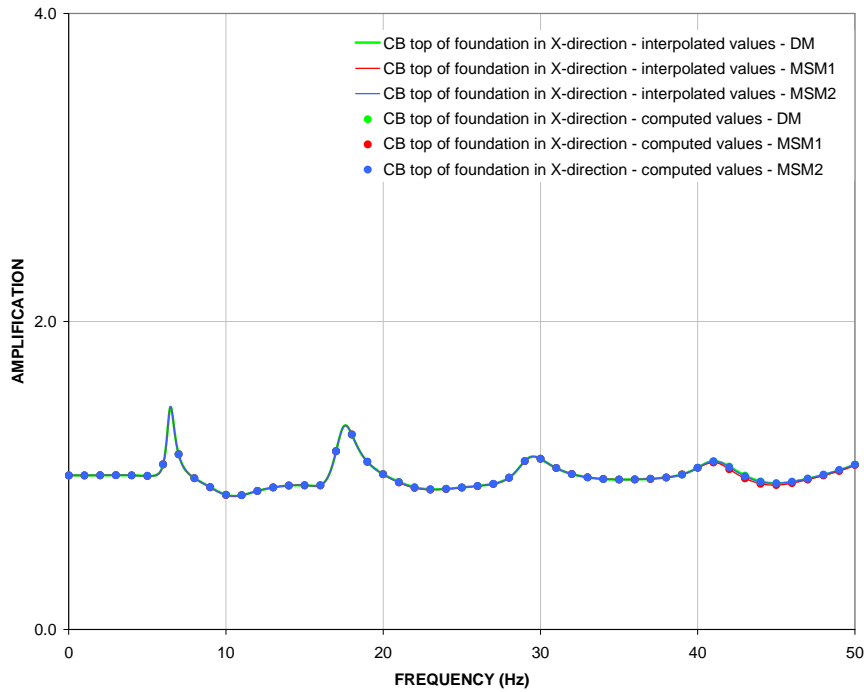
Figure 5: X-Direction DM, MSM1, and MSM2 Transfer Functions CB top of foundation (EL -7.4 m)
