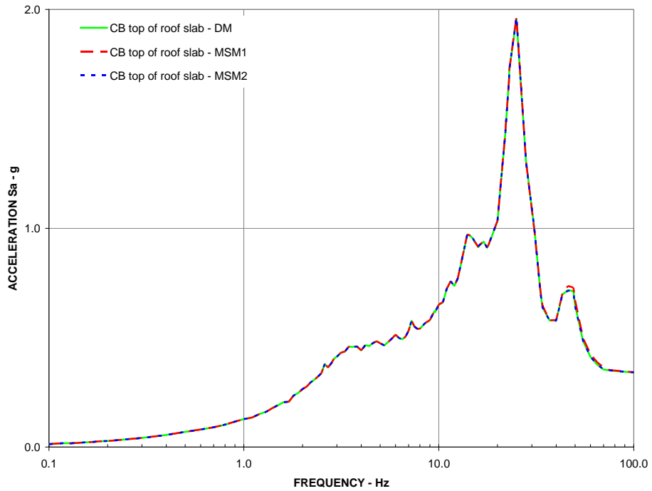
Figure 22: Z-Direction DM, MSM1, and MSM2, 5% Damped Response Spectra CB top of roof slab (EL 13.8 m)
