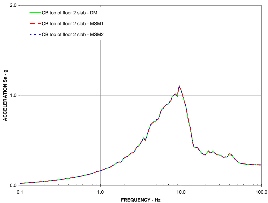
Figure 17: X-Direction DM, MSM1, and MSM2, 5% Damped Response Spectra CB top of floor 2 (EL 4.65 m)
