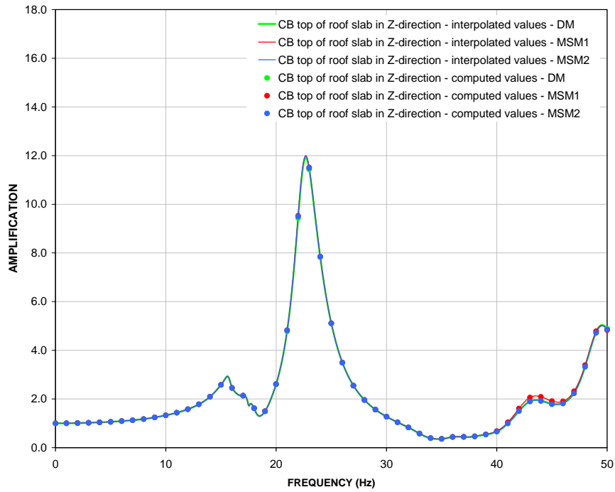
Figure 13: Z-Direction DM, MSM1, and MSM2 Transfer Functions CB top of roof slab (EL 13.8 m)
