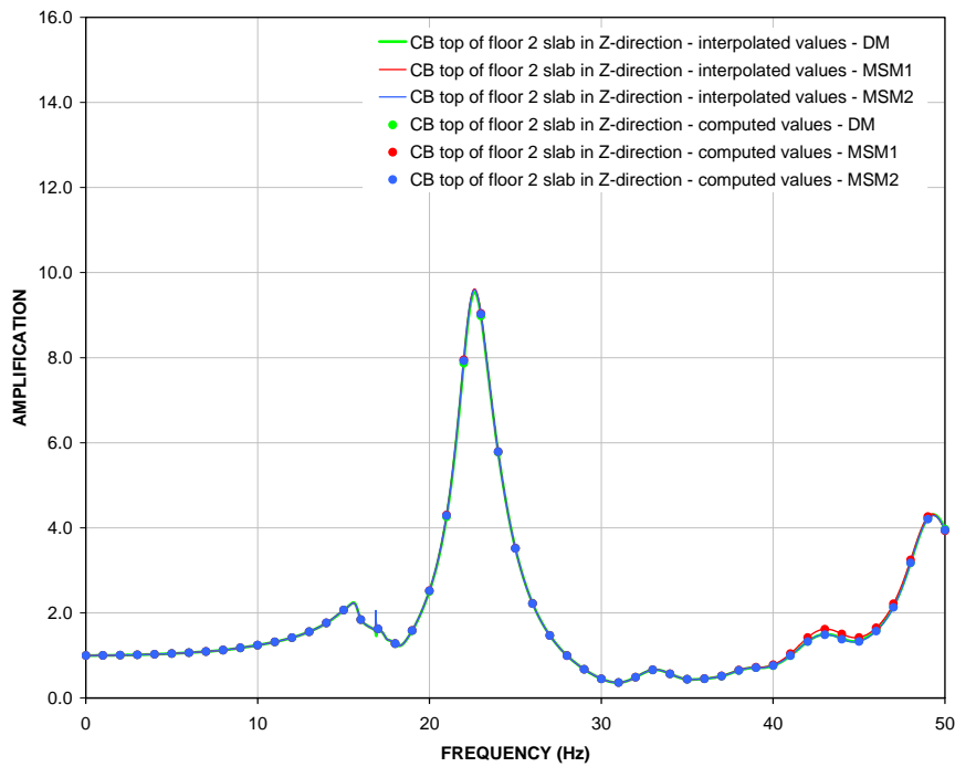
Figure 10: Z-Direction DM, MSM1, and MSM2 Transfer Functions CB top of floor 2 slab (EL 4.65 m)
