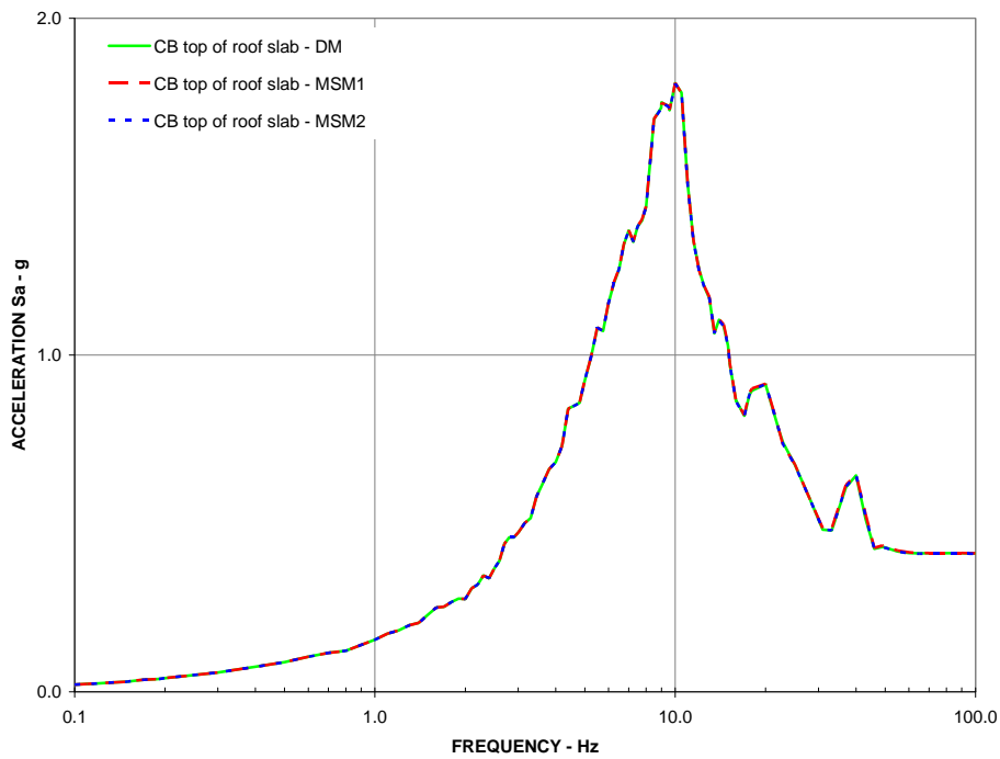
Figure 21: Y-Direction DM, MSM1, and MSM2, 5% Damped Response Spectra CB top of roof slab (EL 13.8 m)
