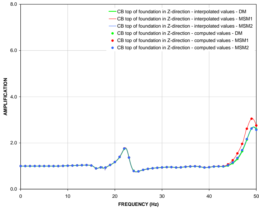
Figure 7: Z-Direction DM, MSM1, and MSM2 Transfer Functions CB top of foundation (EL -7.4 m)
