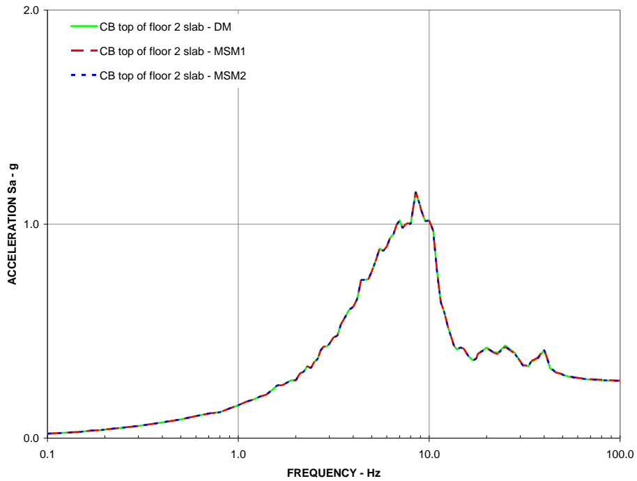
Figure 18: Y-Direction DM, MSM1, and MSM2, 5% Damped Response Spectra CB top of floor 2 (EL 4.65 m)
