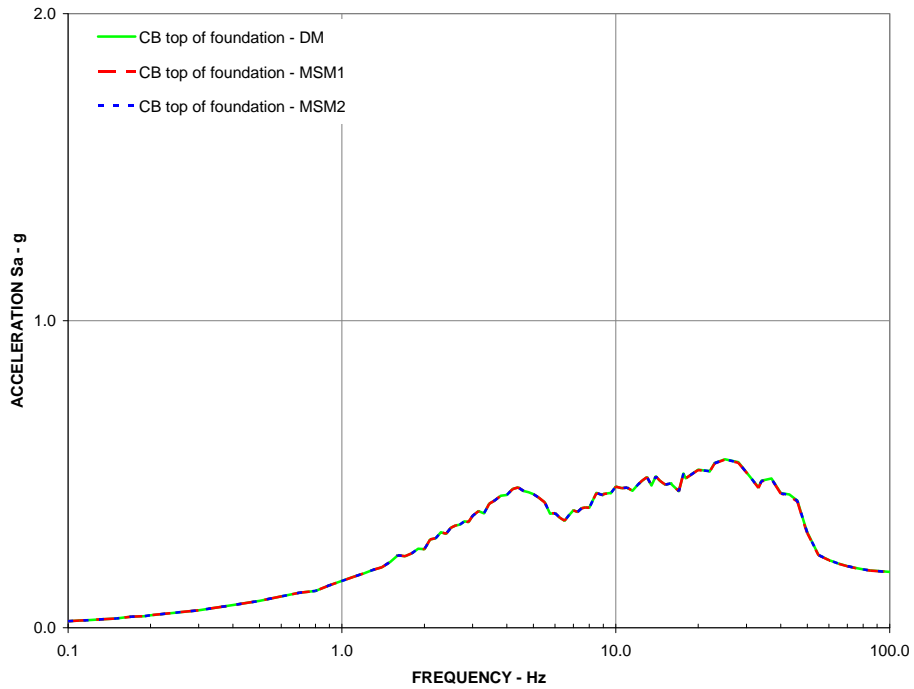
Figure 15: Y-Direction DM, MSM1, and MSM2 5% Damped Response Spectra CB top of foundation (EL -7.4 m)
