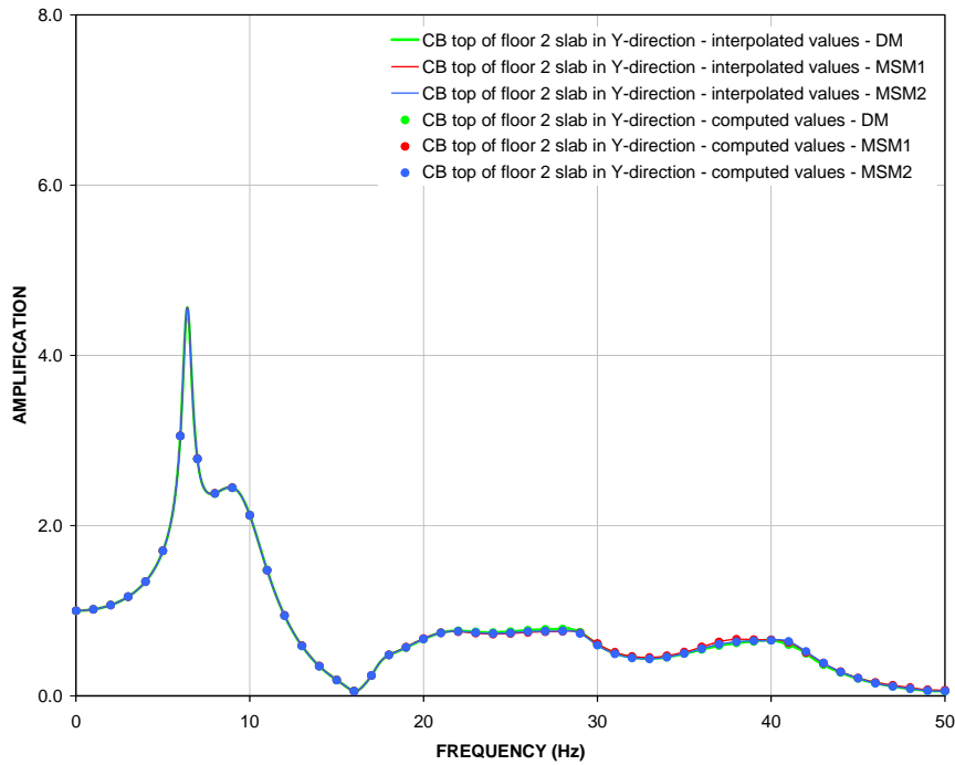
Figure 9: Y-Direction DM, MSM1, and MSM2 Transfer Functions CB top of floor 2 slab (EL 4.65 m)
