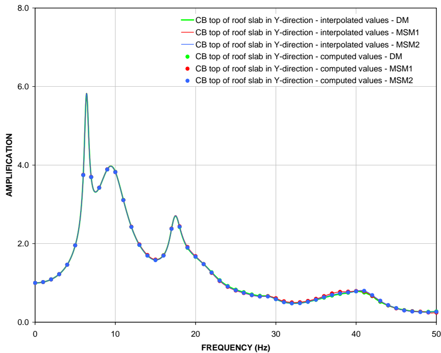
Figure 12: Y-Direction DM, MSM1, and MSM2 Transfer Functions CB top of roof slab (EL 13.8 m)
