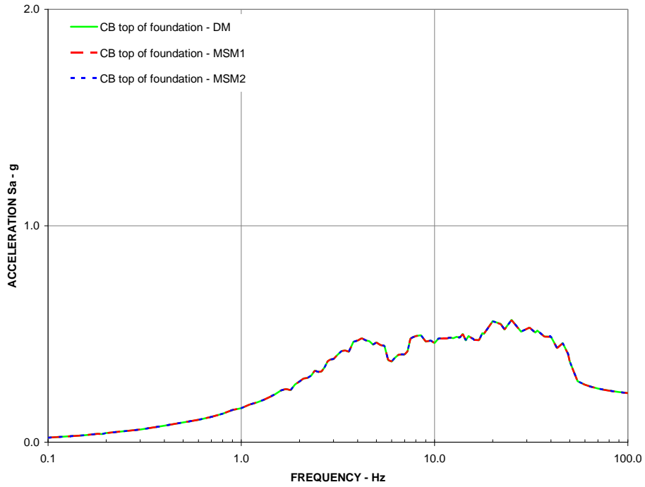
Figure 14: X-Direction DM, MSM1, and MSM2 5% Damped Response Spectra CB top of foundation (EL -7.4 m)
