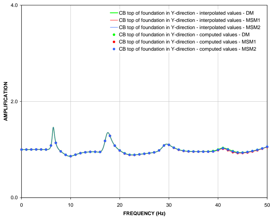
Figure 6: Y-Direction DM, MSM1, and MSM2 Transfer Functions CB top of foundation (EL -7.4 m)
