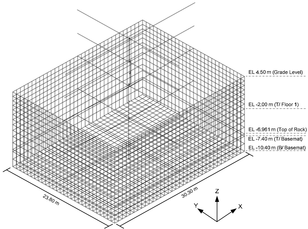
Figure 1: 3-D Isometric View of the CB SASSI2010 Structural Model
