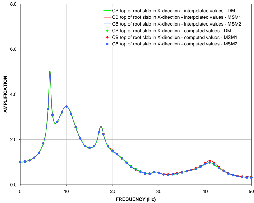
Figure 11: X-Direction DM, MSM1, and MSM2 Transfer Functions CB top of roof slab (EL 13.8 m)
