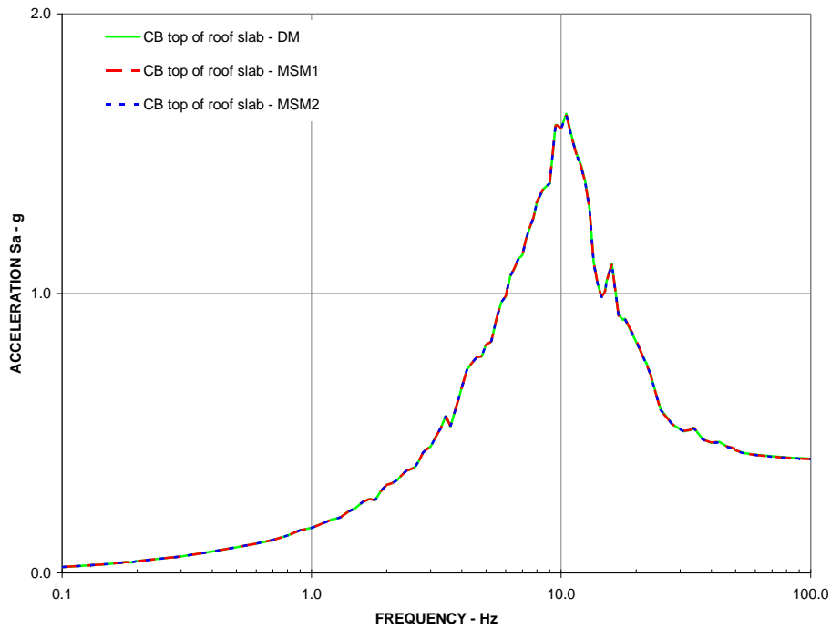
Figure 20: X-Direction DM, MSM1, and MSM2, 5% Damped Response Spectra CB top of roof slab (EL 13.8 m)
